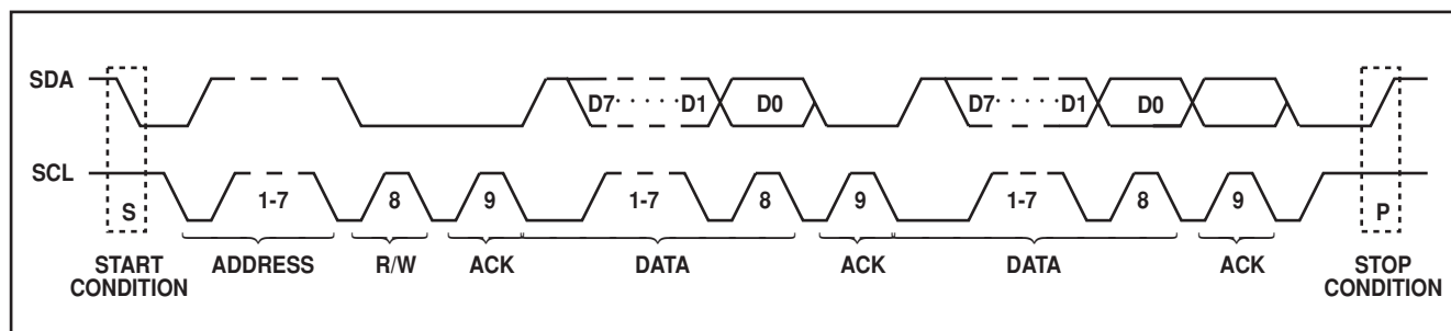
Figure 19 - I²C Data transfer
