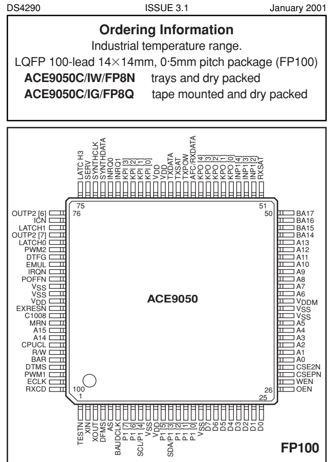
Figure 1 - Pin connections - top view. Pin 1 is identified by moulded spot and by coding orientation. See Table 1 for detailed pin descriptions.
