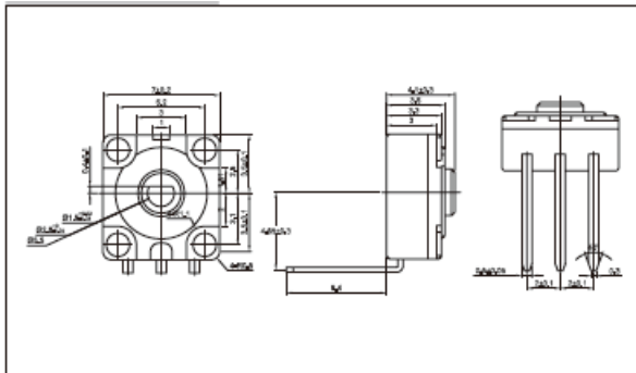
PHS07-01H2 Top Adjust, Terminal Length 6.4mm
