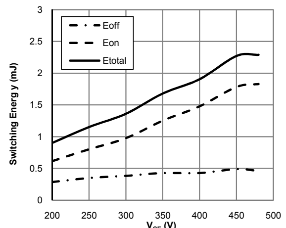
Figure 19: Switching Loss vs. V_{CE} ( T_J=150^\circ\text{C}, V_{GE}=15\text{V}, I_C=30\text{A}, R_g=10\Omega )
