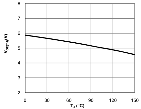
Figure 15: V_{GE(\text{TH})} vs. T_J
