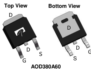
TO252
