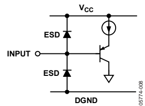
Figure 9. Logic Input
