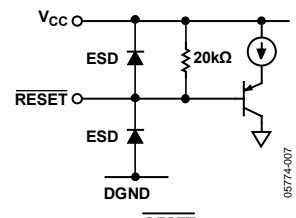
Figure 8. RESET Input
