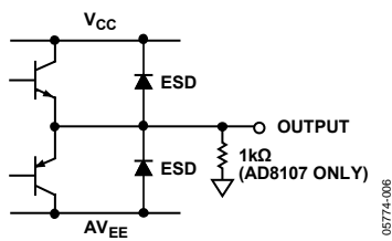
Figure 7. Analog Output
