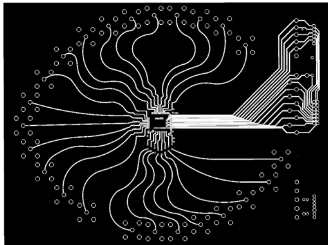
Figure 52. Board Layout (Signal Routing Layer)
