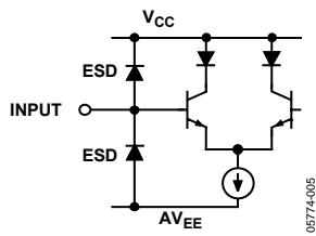
Figure 6. Analog Input
