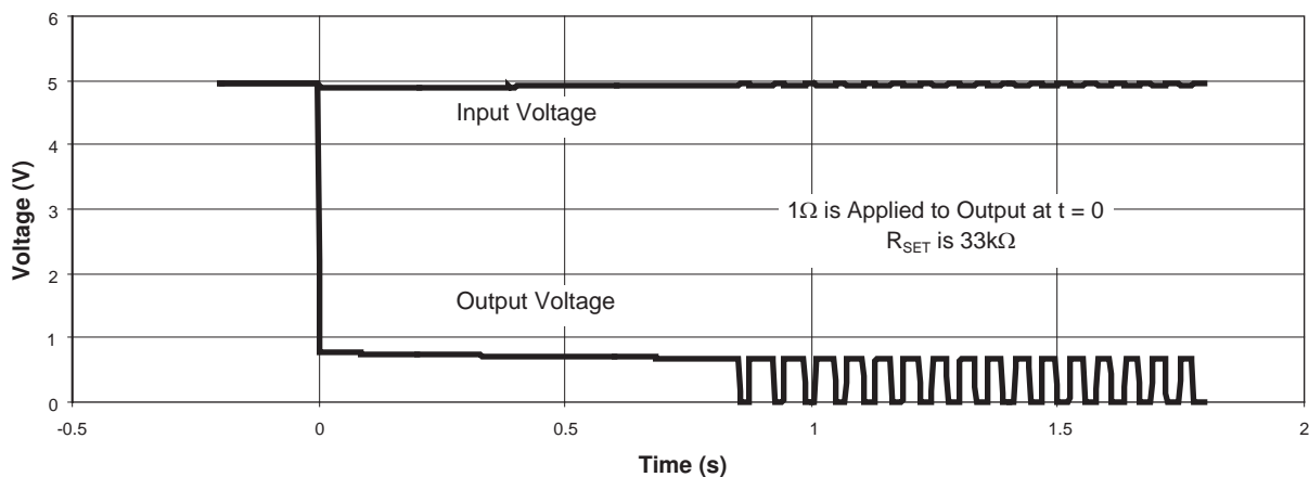
Figure 1: Overload Operation.
