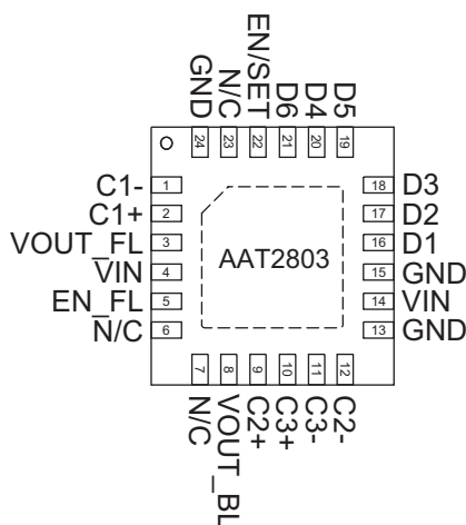
QFN44-24 (Top View)
