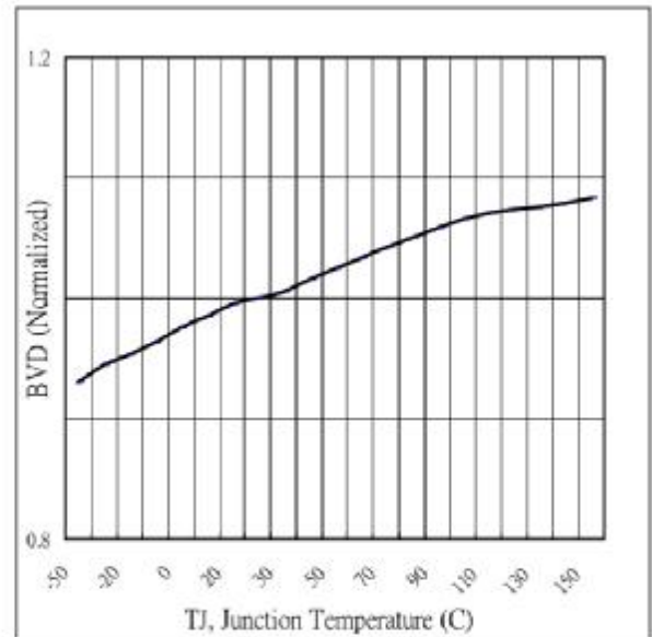
Fig.2 Breakdown Voltage Variation vs. Temperature
