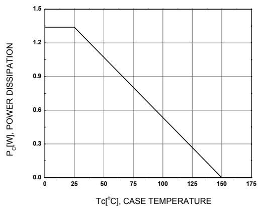
Figure 6. Power Derating
