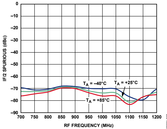
Figure 25. IF/2 Spurious vs. RF Frequency
