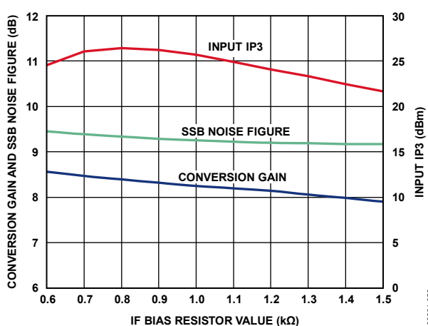
Figure 44. Power Conversion Gain, SSB Noise Figure, and Input IP3 vs. IF Bias Resistor Value
