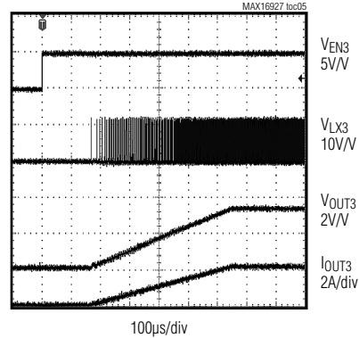
STARTUP BEHAVIOR (BUCK)
