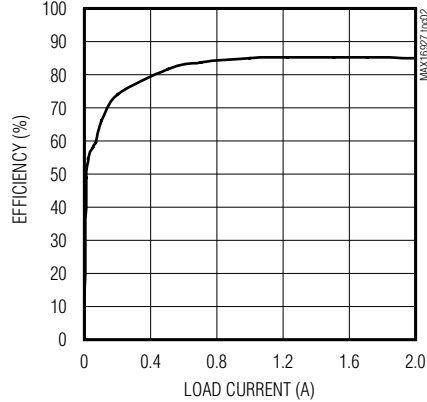
EFFICIENCY vs. LOAD CURRENT (BUCK)
