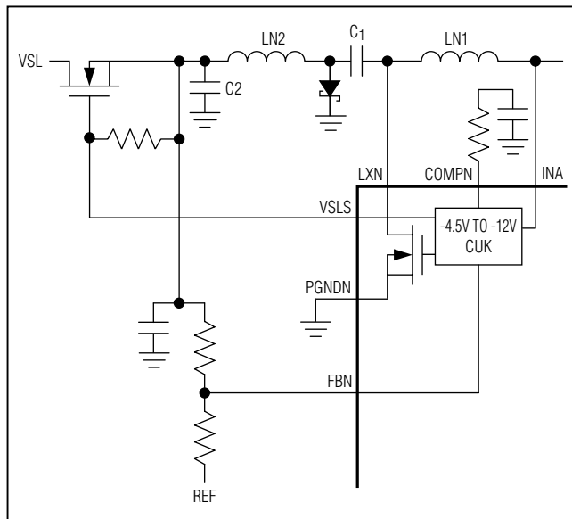
Figure 3. Cuk Converter
