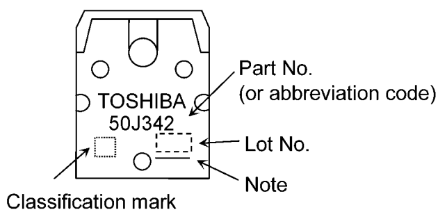
Fig. 7.1 Marking
