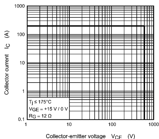
Fig. 8.20 Reverse Bias SOA (Guaranteed Maximum)
