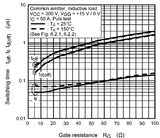
Fig. 8.12 t_{off} , t_r , t_{d(off)} - R_G
