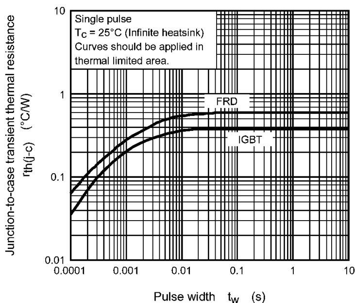
Fig. 8.21 r_{th(j-c)} - t_w (Guaranteed Maximum)
