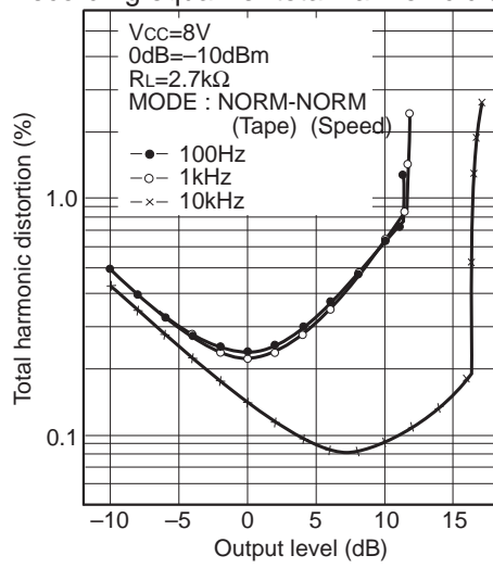
Recording equalizer total harmonic distortion
