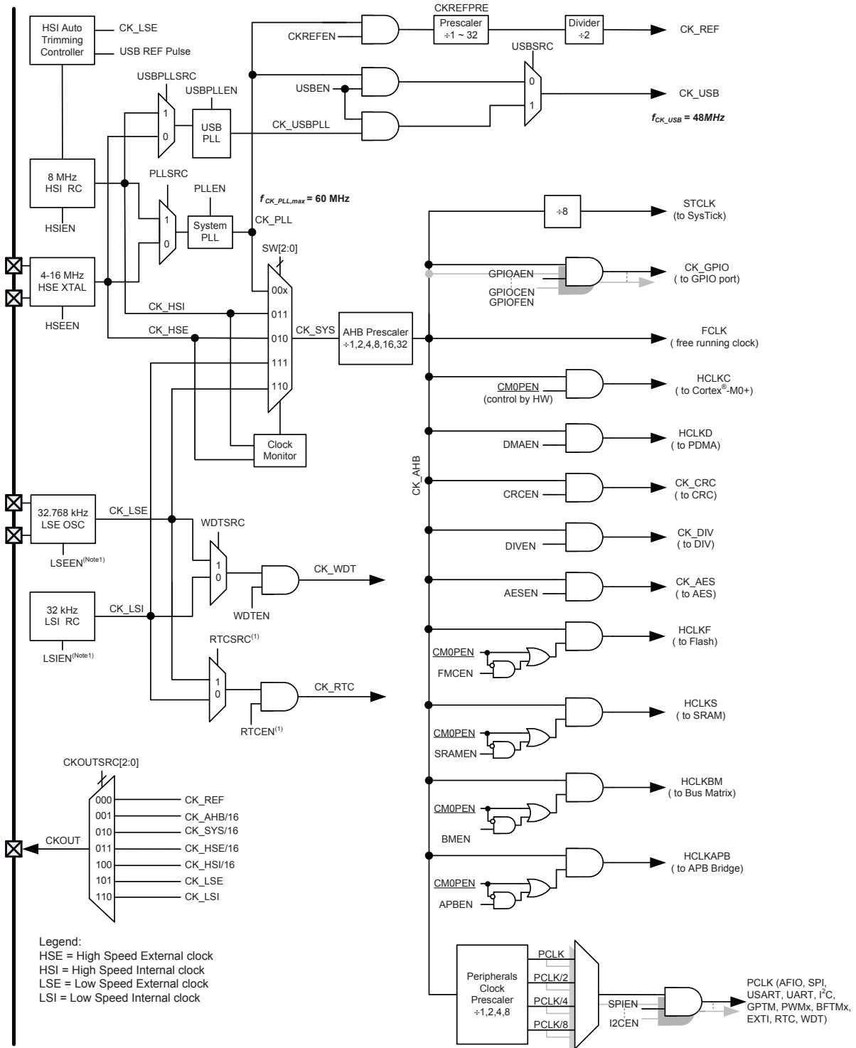
Figure 3. Clock Structure
