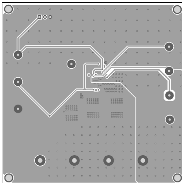
Figure 4: Inner Layer2
