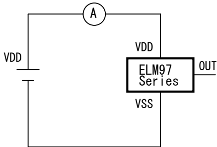
1. Current Consumption
