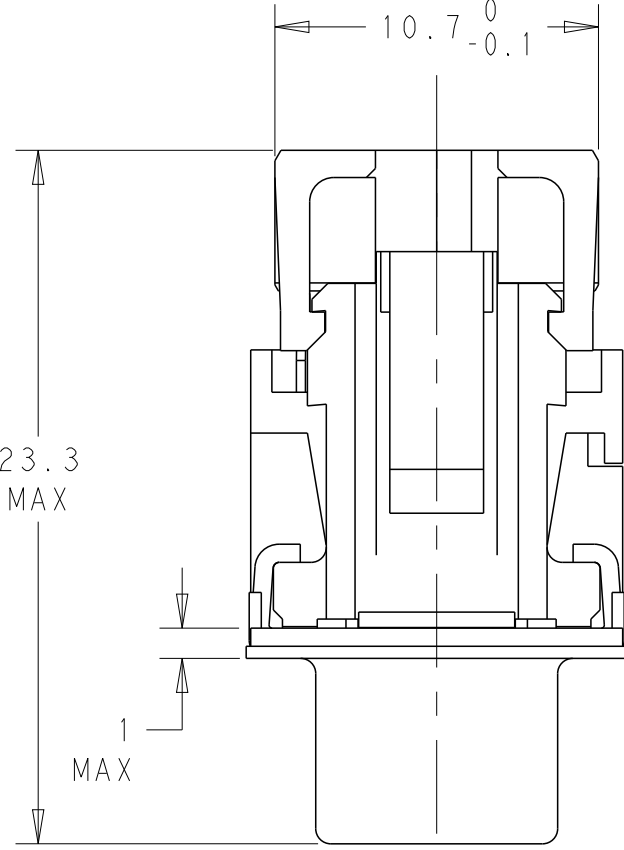
COVER IN PRE-CLAMPED POSITION
