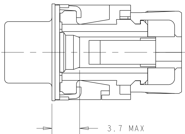
SELF-LOCKING NUT VERSION
