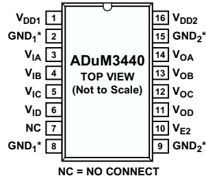
Figure 5. ADuM3440 Pin Configuration
