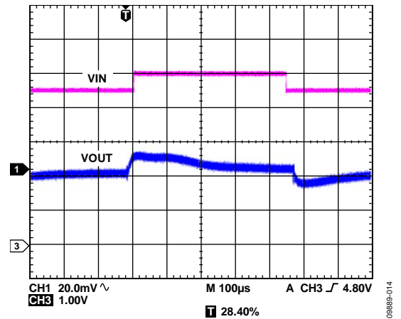
Figure 38. LDO Response to Line Transient, VIN = 4.5 V to 5 V, VOUT3 = 2.8 V
