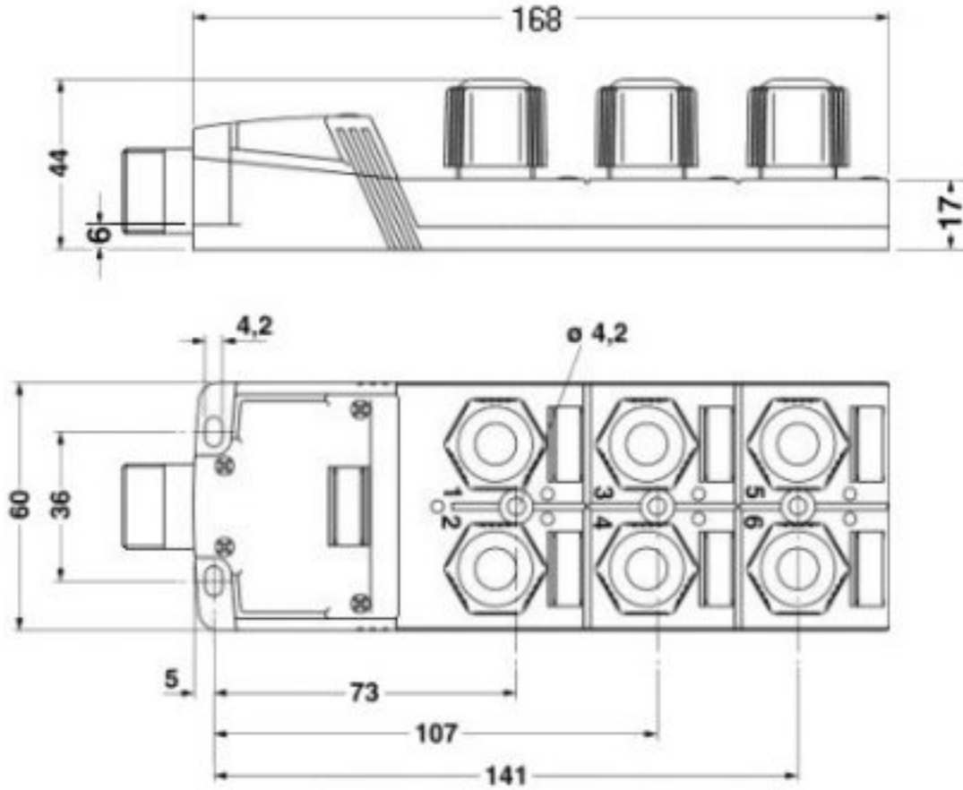
Dimensioned drawing
