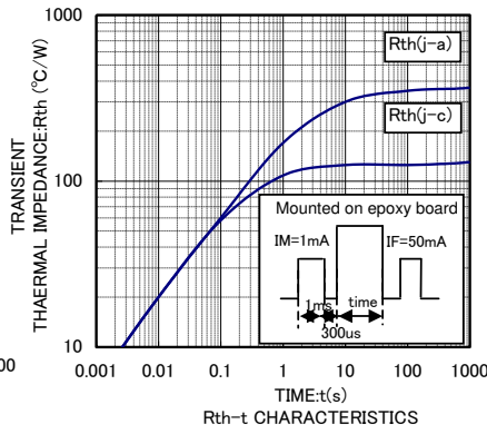
Rth-t CHARACTERISTICS
