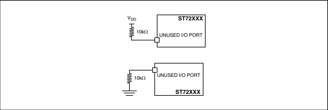
Figure 103. Connecting unused I/O pins
