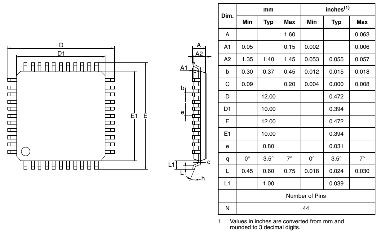
Figure 125. 44-pin low profile quad flat package (10x10)
