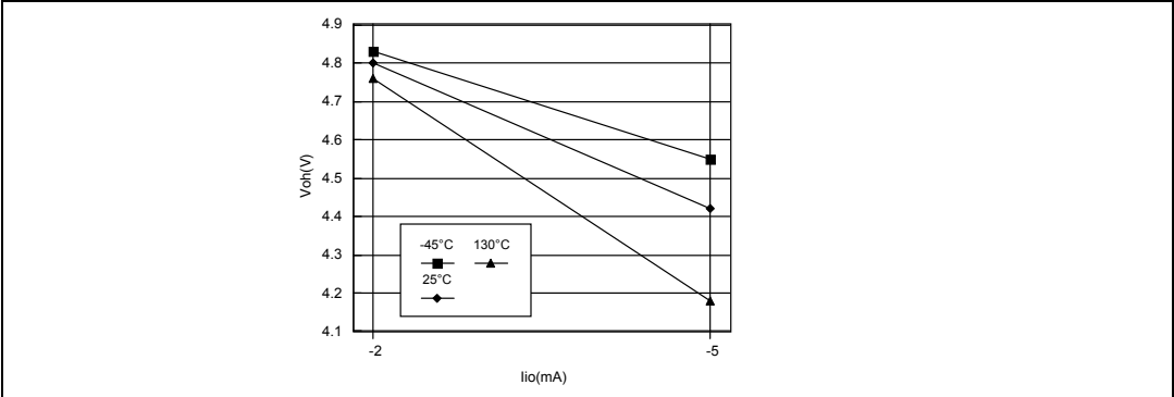
Figure 108. Typical V_{OH} at V_{DD} = 5V
