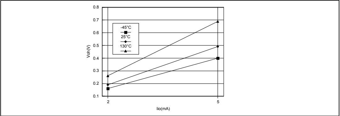
Figure 106. Typical V_{OL} at V_{DD} = 5 \text{ V} (standard)
