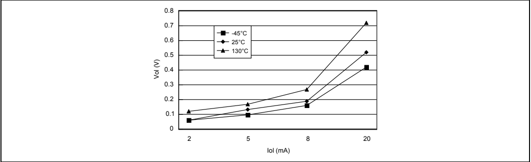
Figure 107. Typical V_{OL} at V_{DD} = 5 \text{ V} (high-sink)
