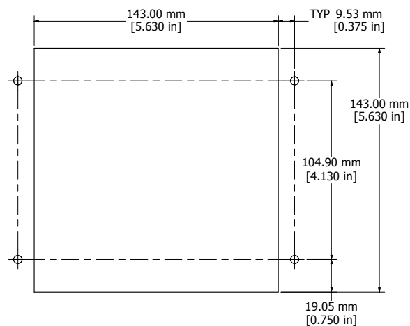
ASSEMBLY CUTOUT
