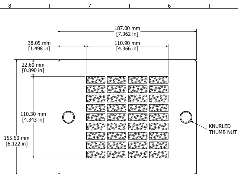
ASSEMBLY - VIEW FROM FRONT
