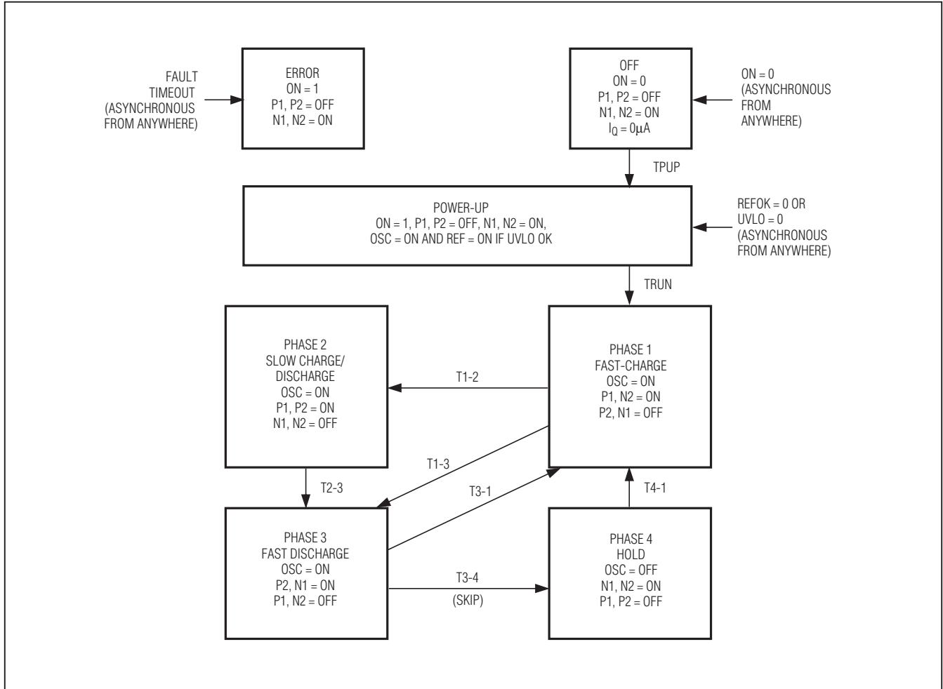
Figure 2. State Diagram
