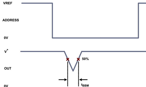
FIGURE 8. BREAK-BEFORE-MAKE DIAGRAM
