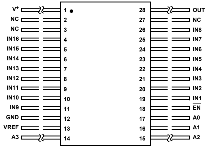
ISL71830SEH (28 LD CDFP) TOP VIEW
