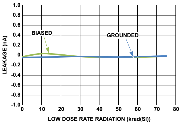
FIGURE 51. I_{D(ON)} ( V^+ = 3.6V , V_{IN} = 3.1V )
