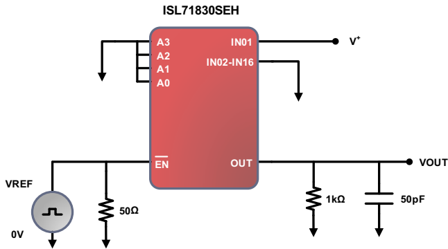
FIGURE 5. TIME TO ENABLE/DISABLE OUTPUT TEST CIRCUIT
