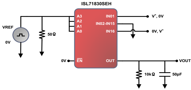
FIGURE 3. ADDRESS TIME TO OUTPUT TEST CIRCUIT
