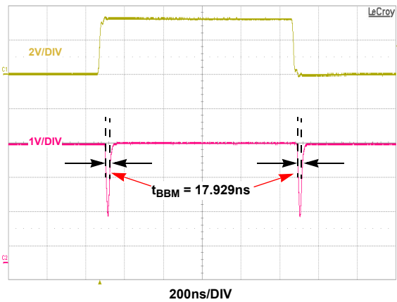
FIGURE 21. BREAK-BEFORE-MAKE DELAY
