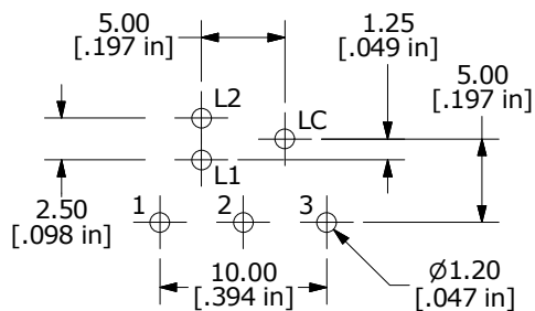
PCB MOUNTING
