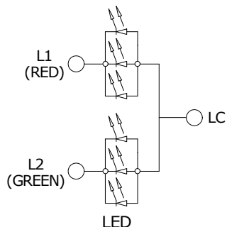
CIRCUIT LAYOUT
