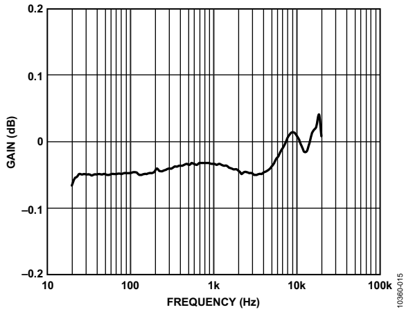
Figure 16. Frequency Response, PVDD = 3.0 V
