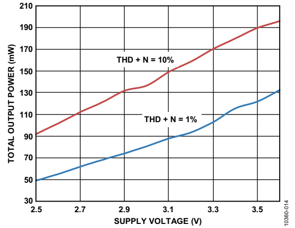
Figure 18. Output Power vs. Supply Voltage, R_L = 16 \Omega
