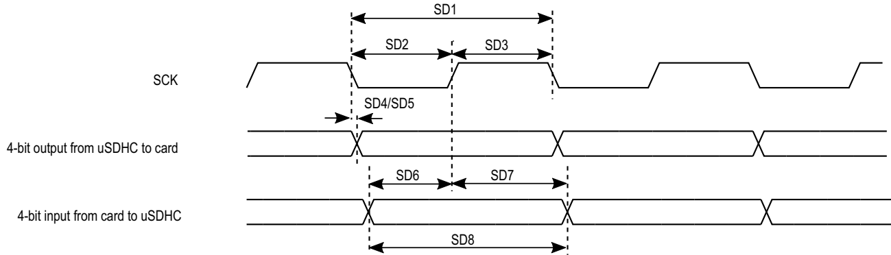
Figure 20. SDR50/SDR104 Timing
