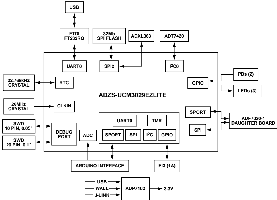
Figure 2. ADuCM3029 EZ-KIT (Mother Board for the ADF7030-1 Daughter Board) Block Diagram
