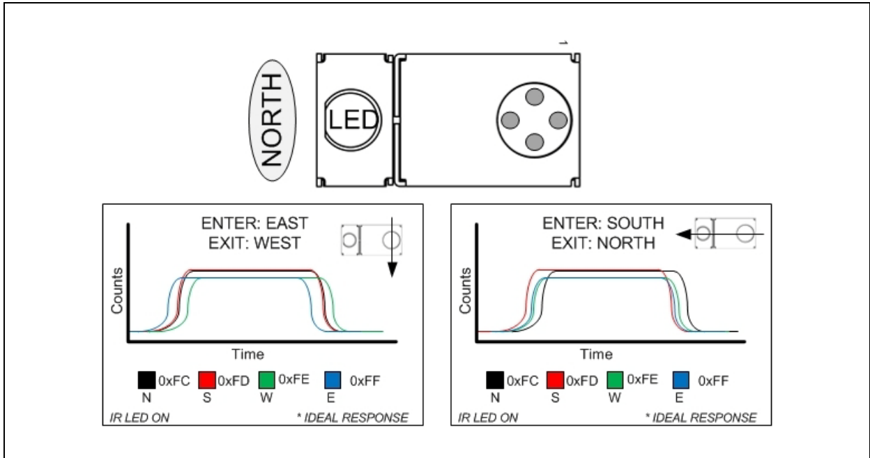
Figure 37: Directional Orientation
