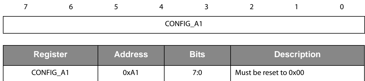
Figure 65: Configuration Register A1
