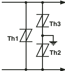
Figure 17. MULTI-POINT PROTECTION
