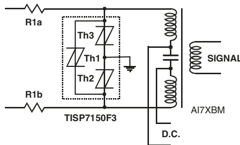
Figure 22. ISDN Protection
