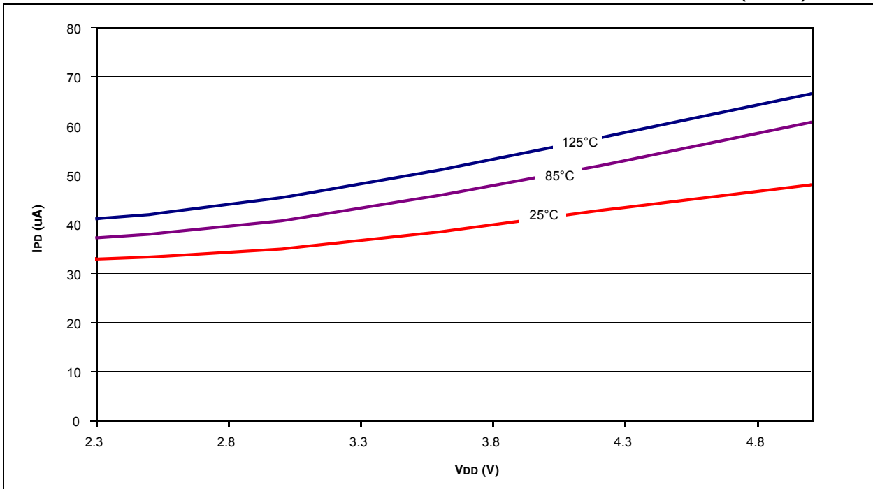
FIGURE 27-14: MEMLOW TYPICAL IPD FOR DIGITAL-TO-ANALOG CONVERTER ( CV_{REF} )
