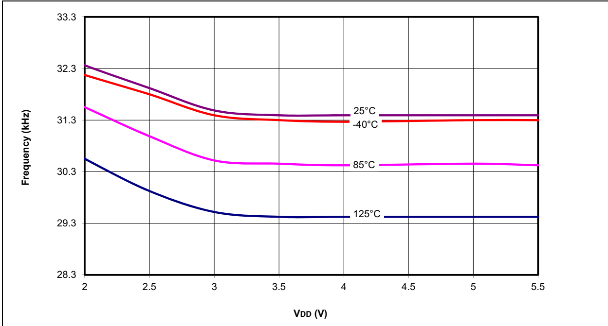
FIGURE 27-25: MEMLOW TYPICAL LF-INTOSC FREQUENCY (MAX./MIN. = 31.25 kHz ± 15%)
