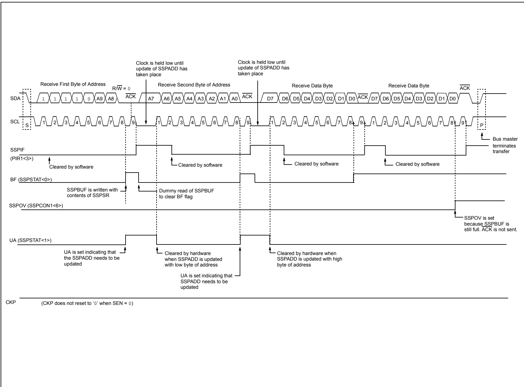
FIGURE 14-10: I 2 C SLAVE MODE TIMING WITH SEN = 0 (RECEPTION, 10-BIT ADDRESS)
