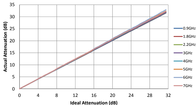
Figure 11. 0.5 dB Step, Actual vs. Frequency
