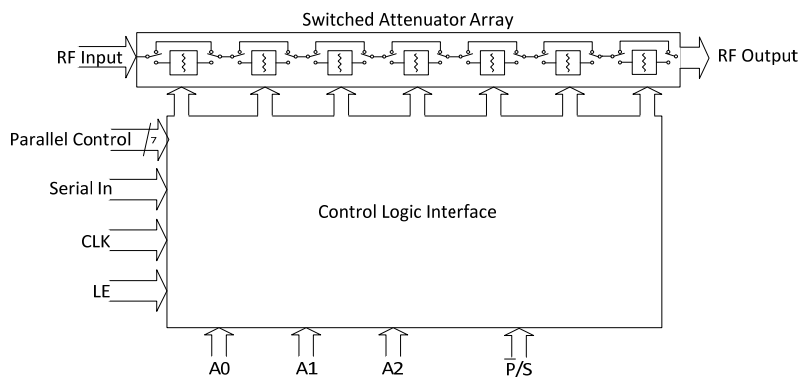
Figure 1. Functional Diagram
