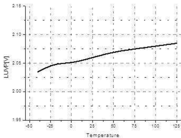
LUV vs. Temp
