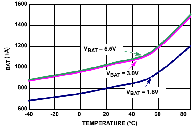
FIGURE 4. I_{BAT} vs TEMPERATURE ( V_{DD} = 0V )
