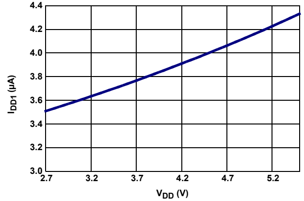
FIGURE 6. I_{DD1} vs V_{DD}
