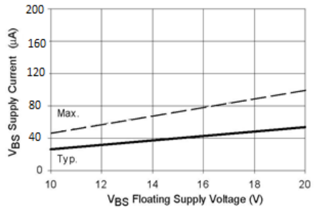
Figure 17B. V_{BS} Supply Current vs. Supply Voltage
