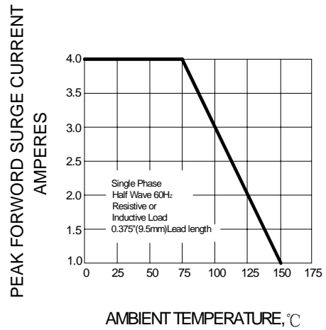
FIG.5-FORWARD DERATING CURVE
