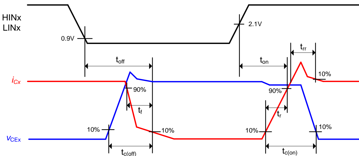
Figure 10: Switching times definition
