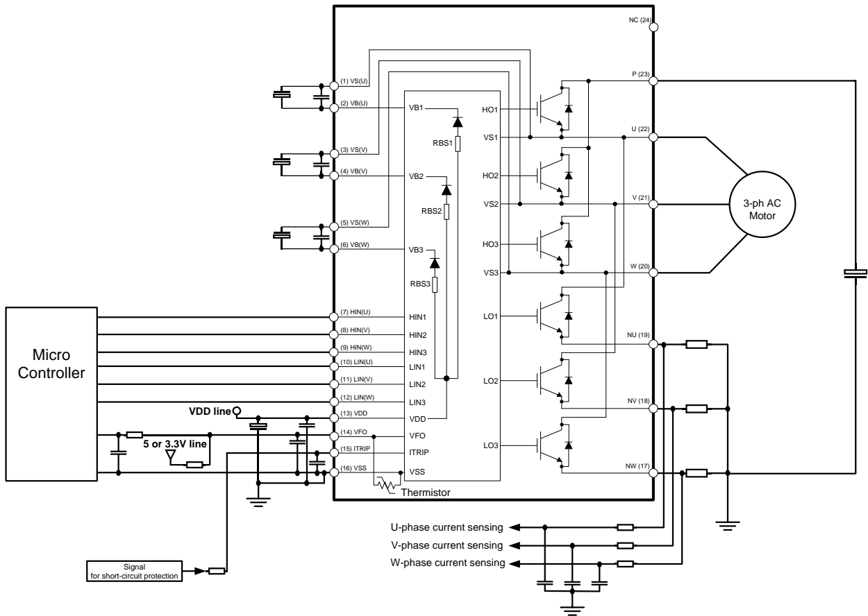
Figure 9: Application circuit
