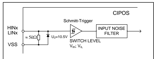
Figure 3: Input pin structure
