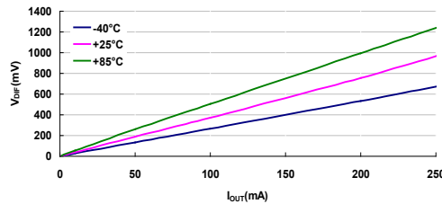
Dropout Voltage: HT7333-3
