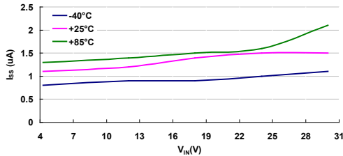
I_{SS} vs V_{IN} : HT7333-3 ( I_{OUT}=0mA )
