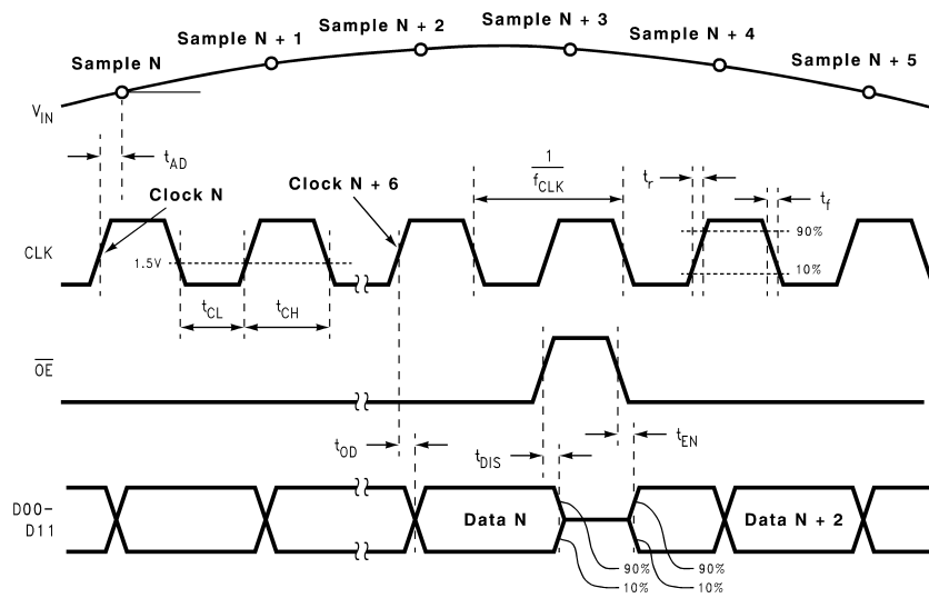
Figure 1. Output Timing
