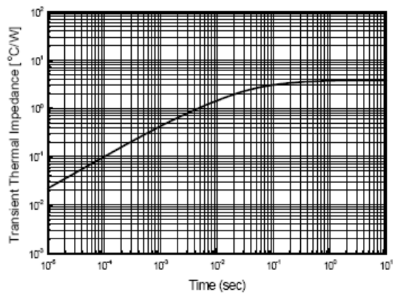
Fig.4 Thermal Response
