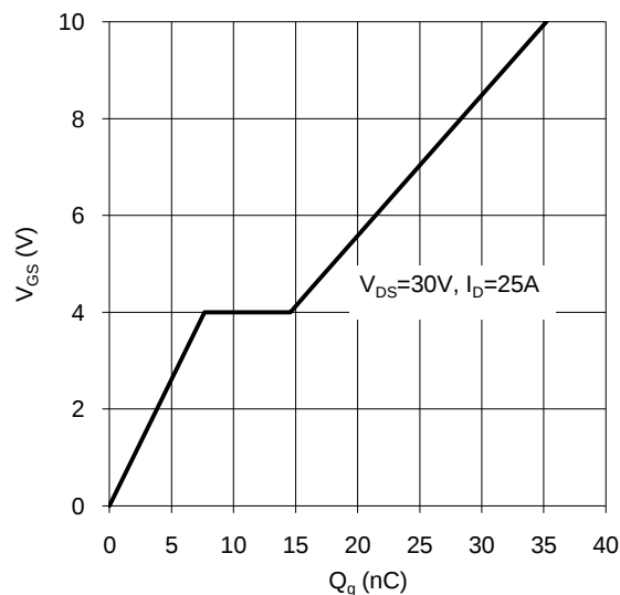
Figure 12. Gate Charge
