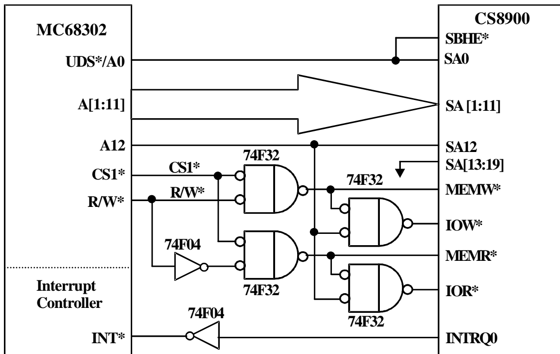
Figure 3. Connection of CS8900A to MC68302
