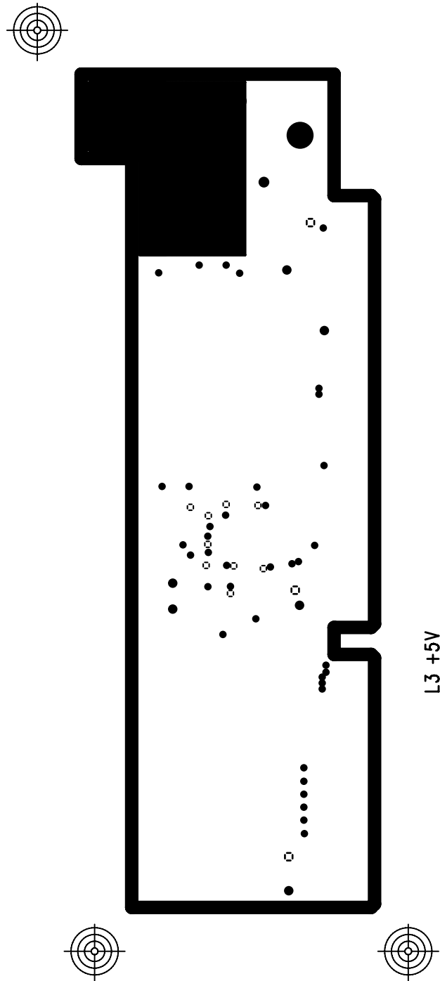
Figure 28. +5V Plane of four-layer board
