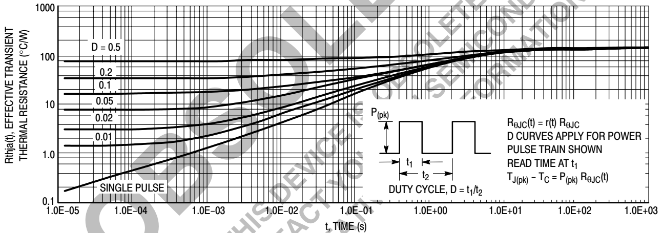
Figure 16. Thermal Response
