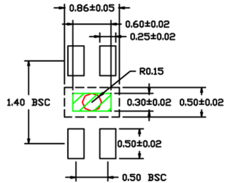
RECOMMENDED LAND PATTERN NOTE: 4, 5
