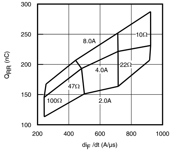
Fig. 21 - Typ. Diode Q_{RR} vs. di_F/dt
