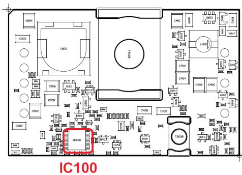
Fig 17: Conformal coating will be applied over IC100 for SQE48T40050 NGALG to pass Telcordia GR-63-CORE Mixed Flow Gas Test
