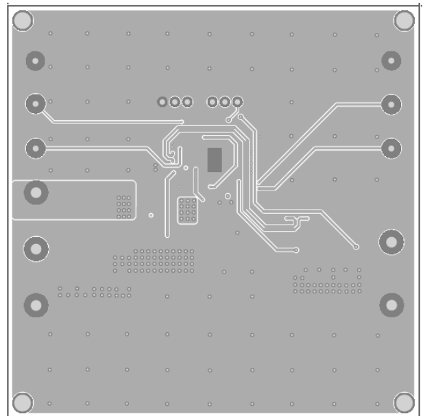
Figure 4—Inner Layer
