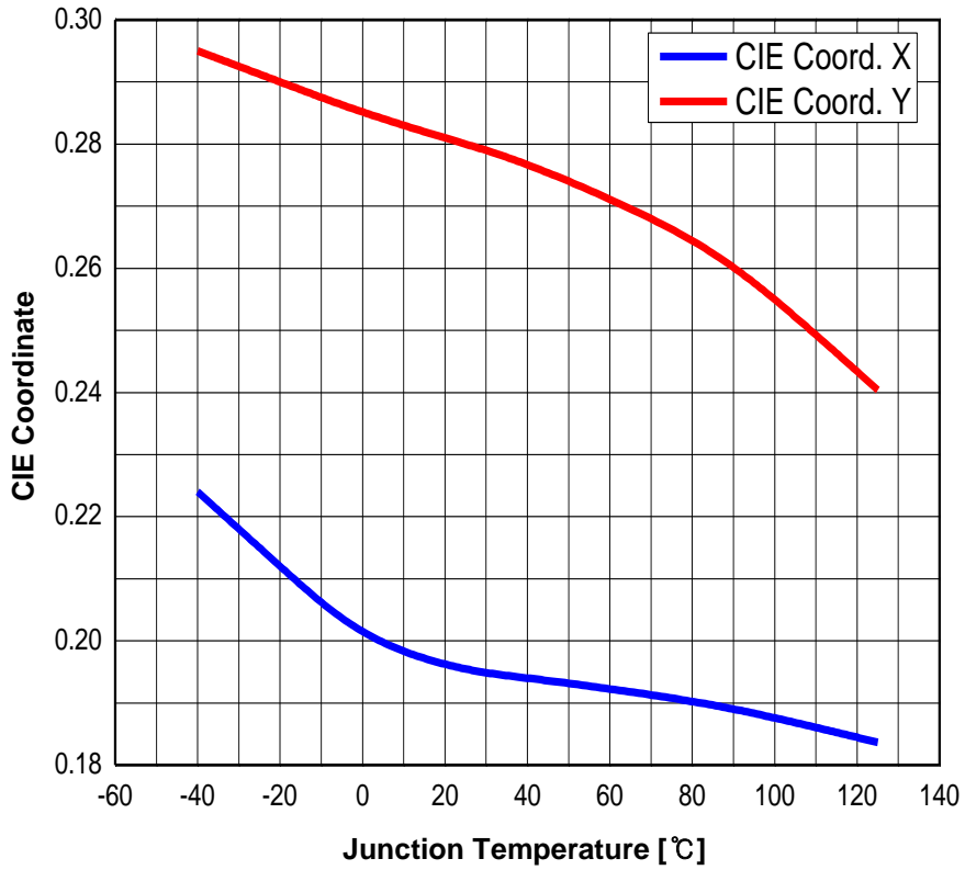
Fig 8. Chromaticity Coordinate vs. Junction Temperature, I_F = 20\text{mA}
