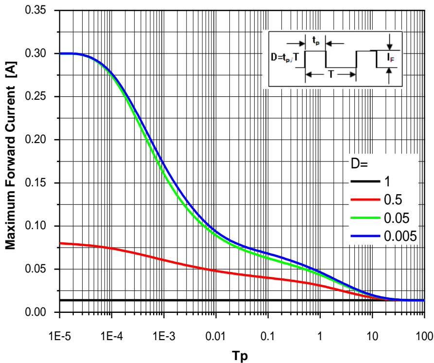
Fig 12. Maximum Forward Current vs. Duty Ratio, T_a = 85^\circ\text{C}
