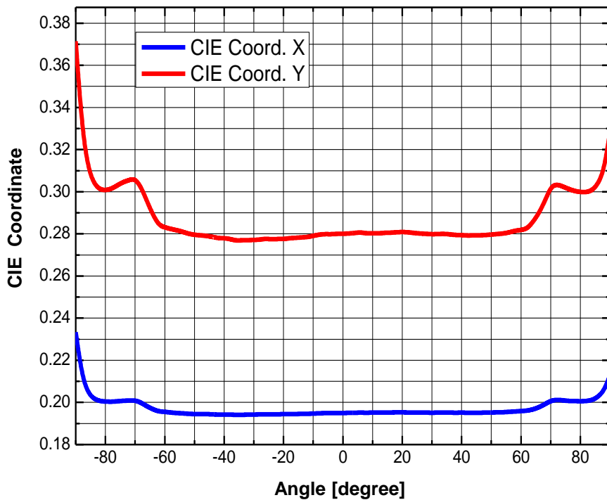
Fig 10. Color. vs. Viewing Angle, T_a = 25^\circ\text{C} , I_F = 20\text{mA}
