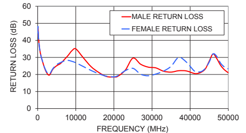
BLK-V54+ RETURN LOSS
