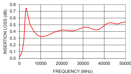
BLK-V54+ INSERTION LOSS
